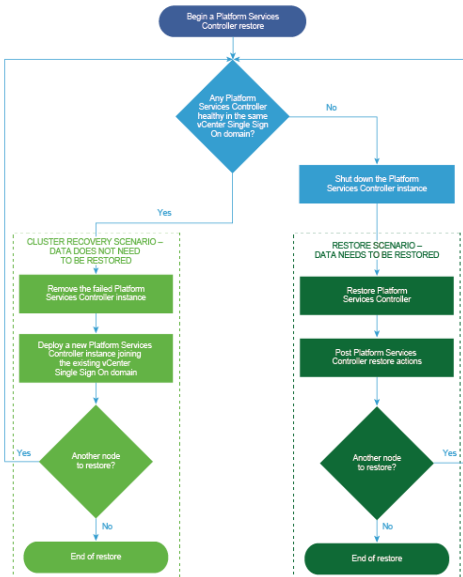
Figure 9. PSC restore workflow
