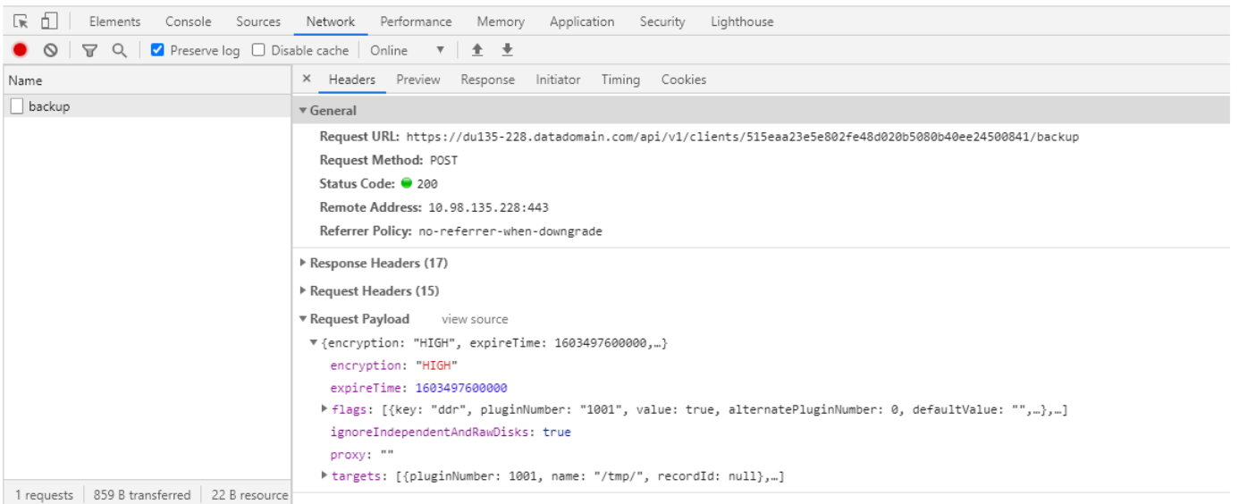
Figure 26. REST API Request
