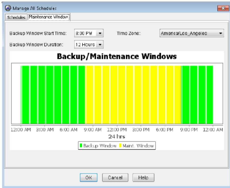
Figure 16. Default backup and maintenance windows
