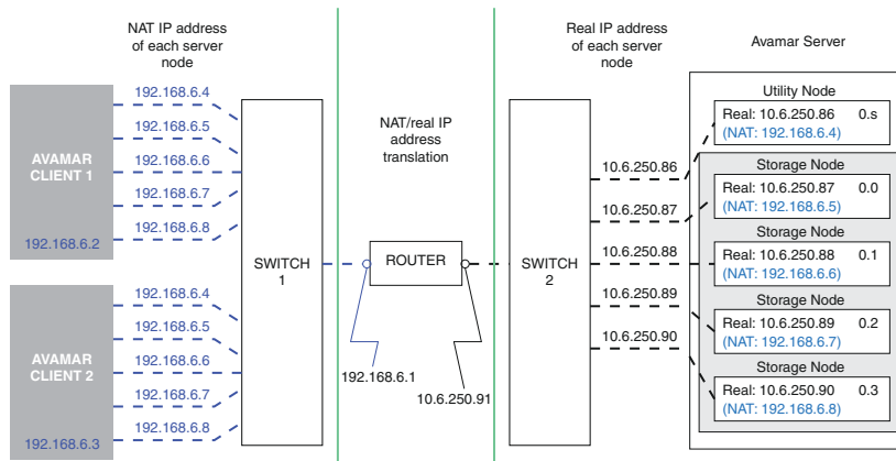
Figure 20. Multi-node server configuration with NAT
