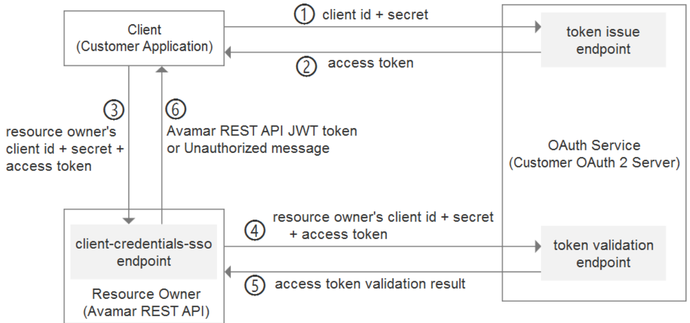
Figure 27. Integration Process Flow
