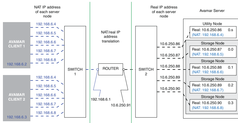
Figure 14. Multi-node server configuration with NAT
